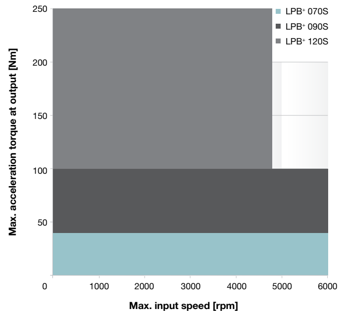
LPB + Generation 3 (example for i = 5 ) For applications in cyclic operation ( ED \leq 60\% )
