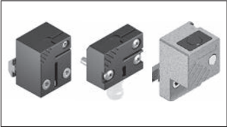
Switch brackets SH 2/U, SH 2/UV, SH 2/U-H 8-98
