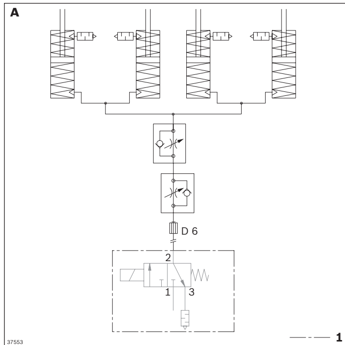
Circuit diagram for unit with pneumatic equipment for 2 positions PN = 2, BG 3
