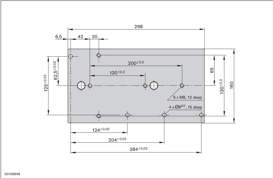
Drilling plan PE 2/XP, upper part, BG 2
