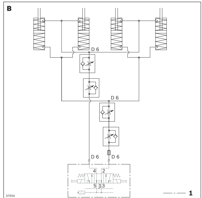
Circuit diagram for unit with pneumatic equipment for 3 positions PN = 3, BG 3
