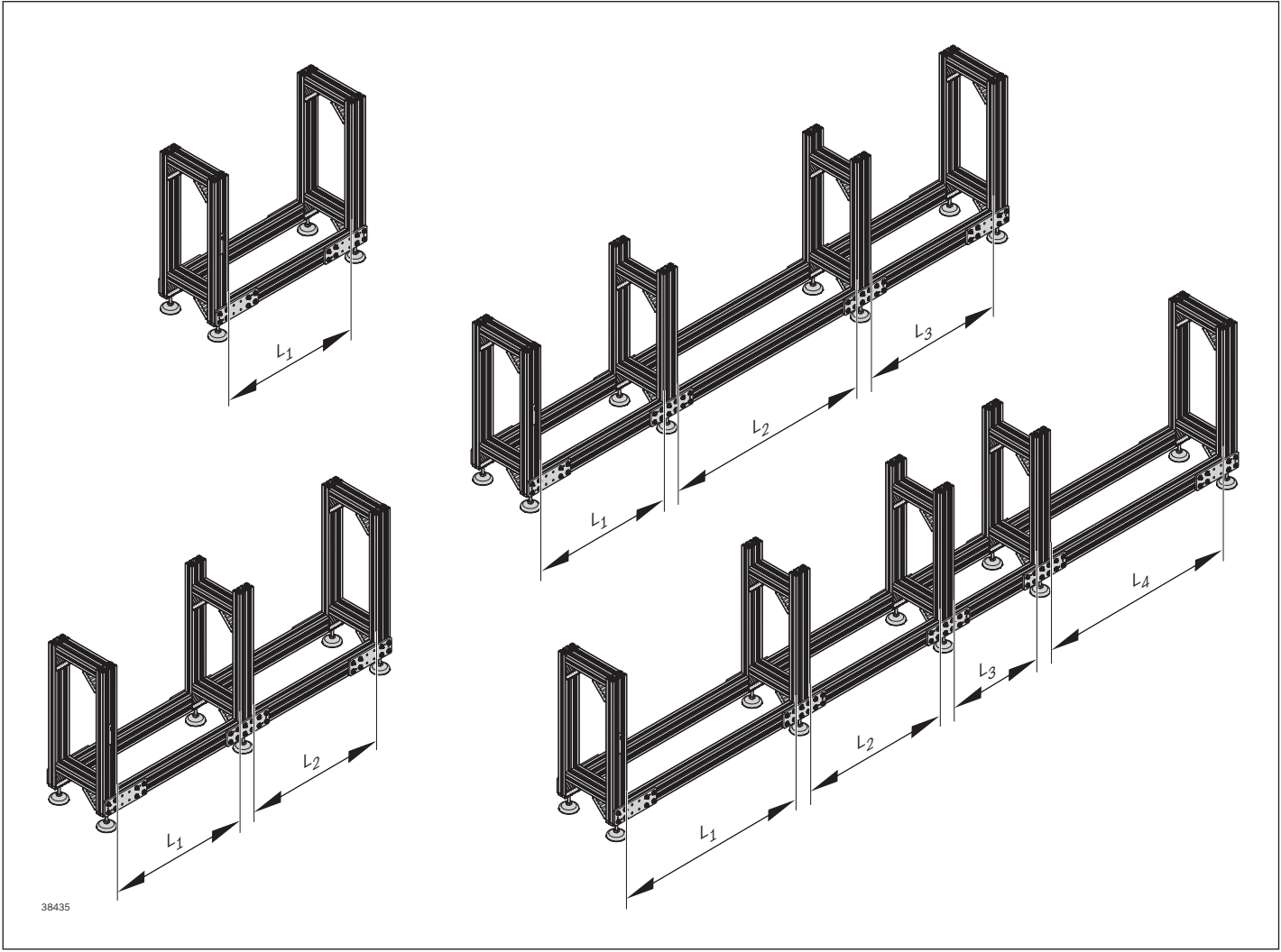
Lengths of longitudinal connectors LV 2
