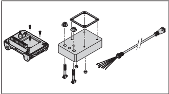
Connection unit Attachment kit Connection cable 8-124
