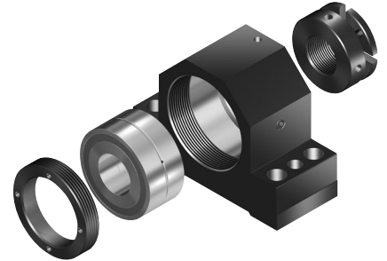
Pillow block unit SEB-F assembly
