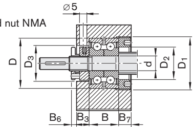
LGN-B-... with slotted nut NMA
