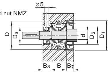
LGN-B-... with slotted nut NMZ
