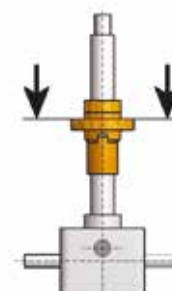
„Direction of loading, compressive“ (towards the gearbox)
