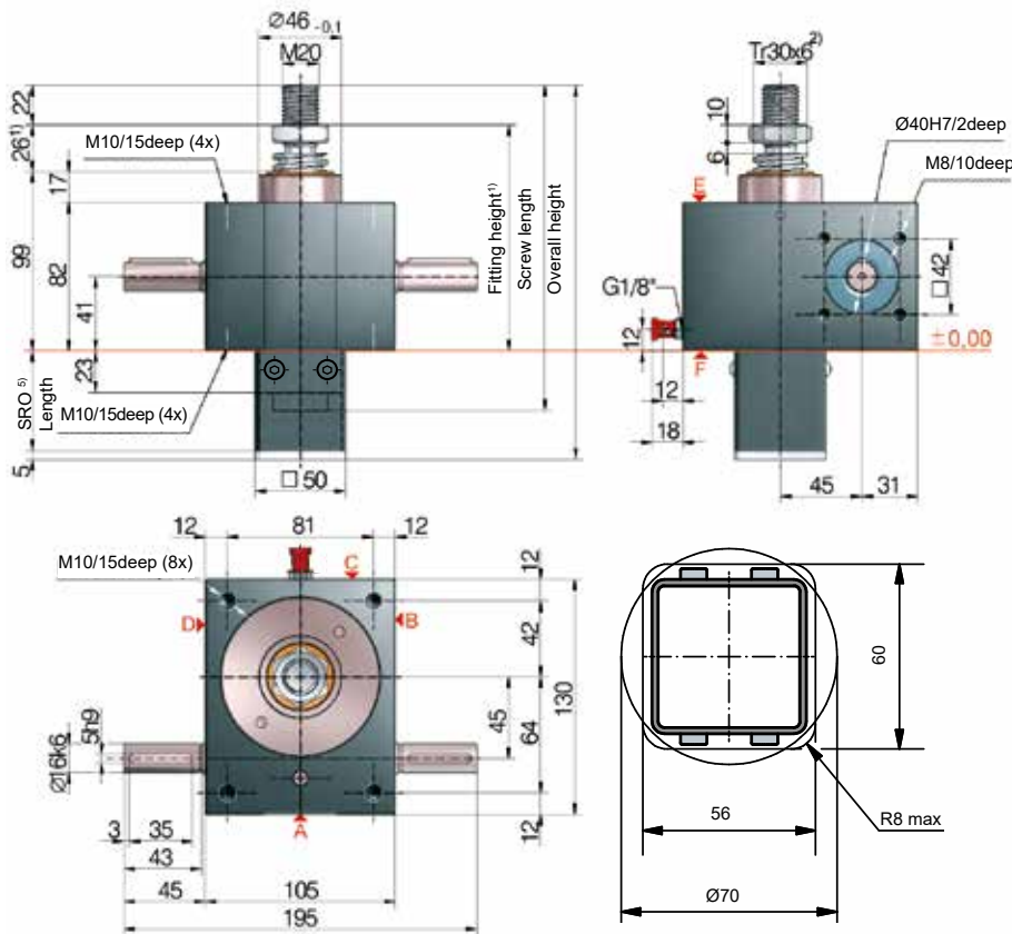
Opening for protective tube square and round
