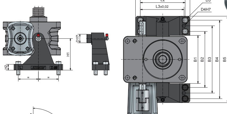
Bearing mount LB (35 - 350)
