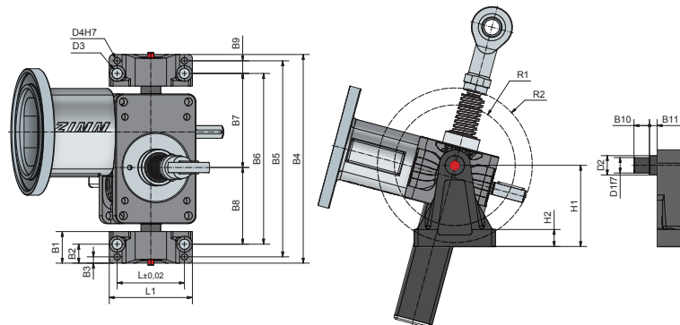
Pivot mounts LB (5 - 25)
