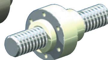
Greaseless nut FFDM - Specially suitable for dry running (such as textiles, foodstuffs, chemicals,...) - Bellows can be attached both sides - Reinforced with a stainless steel washer
