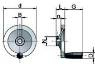
Handwheel HR
