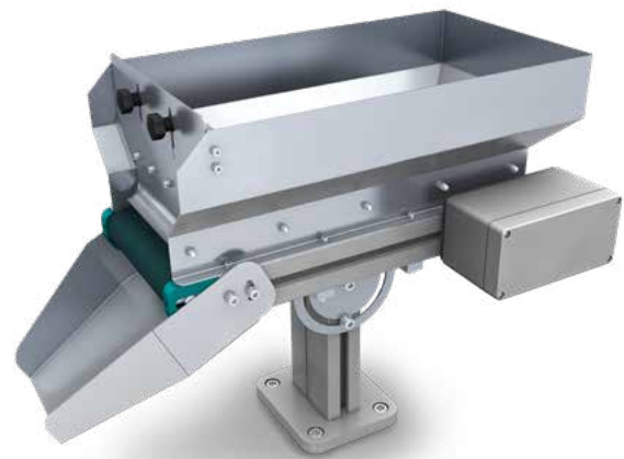
Figure: Custom design – hopper conveyor
