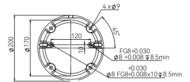
EC64-19 base top view
