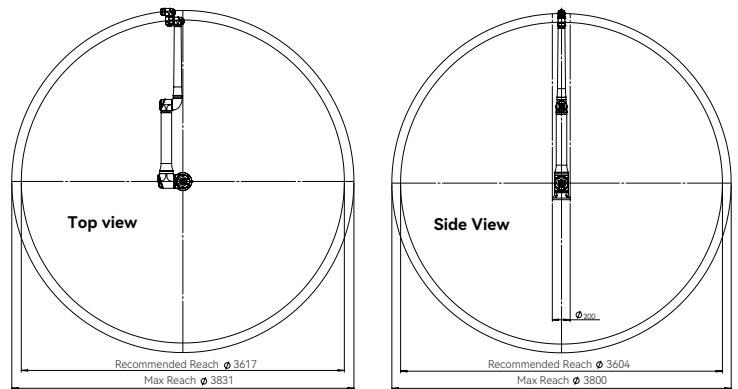
EC64-19 working range diagram
