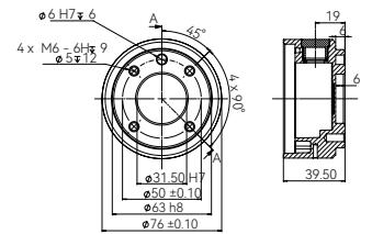
EC64-19 end flange
