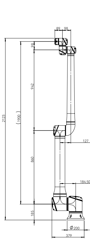
EC64-19 external dimensional drawing
